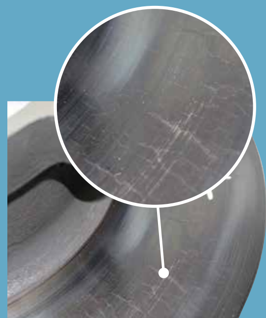
SOLID BRAKE DISC AFTER 15 BRAKE CYCLES Minimal heat crazing but no cracks
